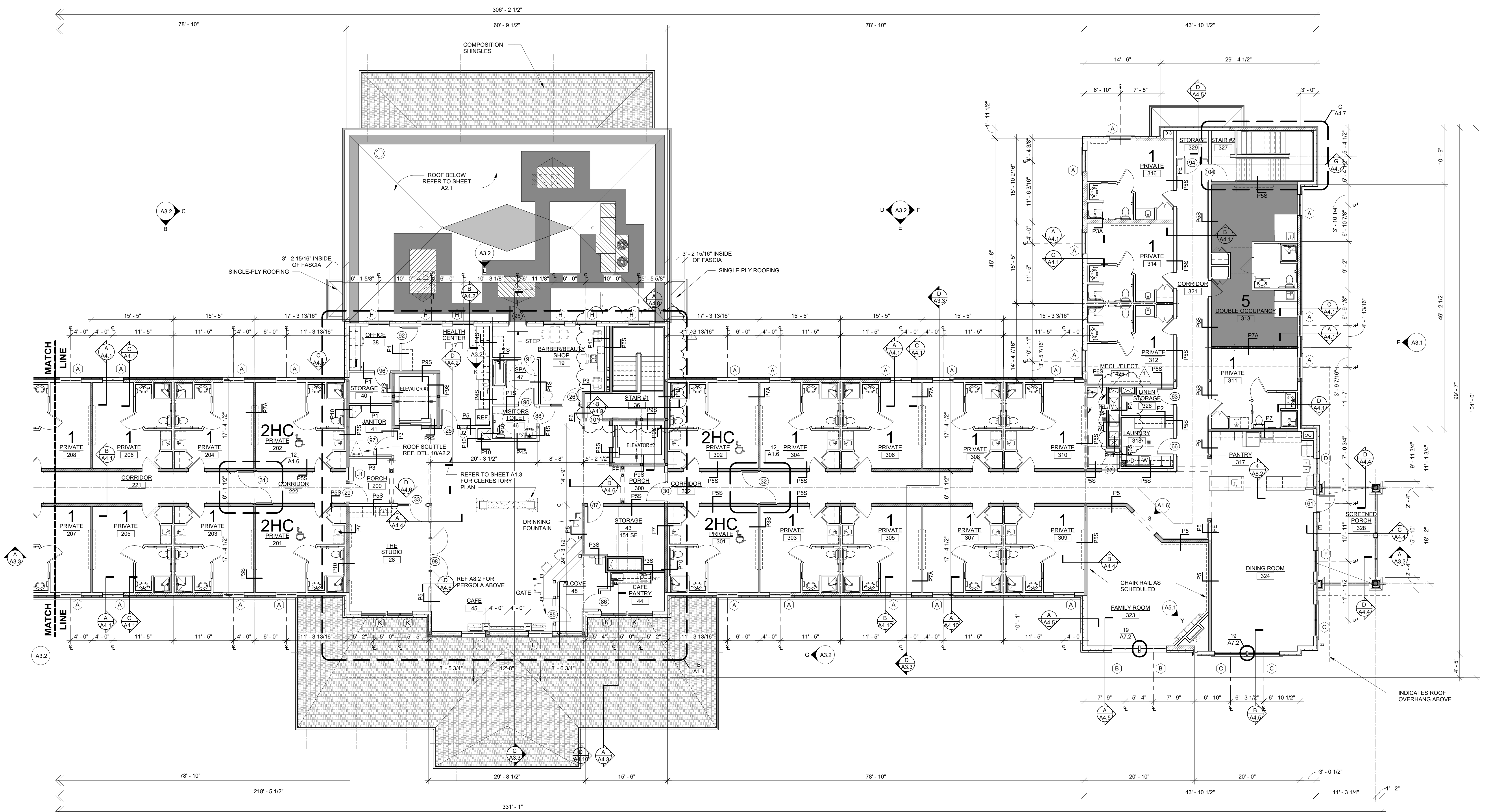
A 2nd FLOOR PLAN - AREA A 1/8" = 1'-0" 0' 4' 8' 16'
