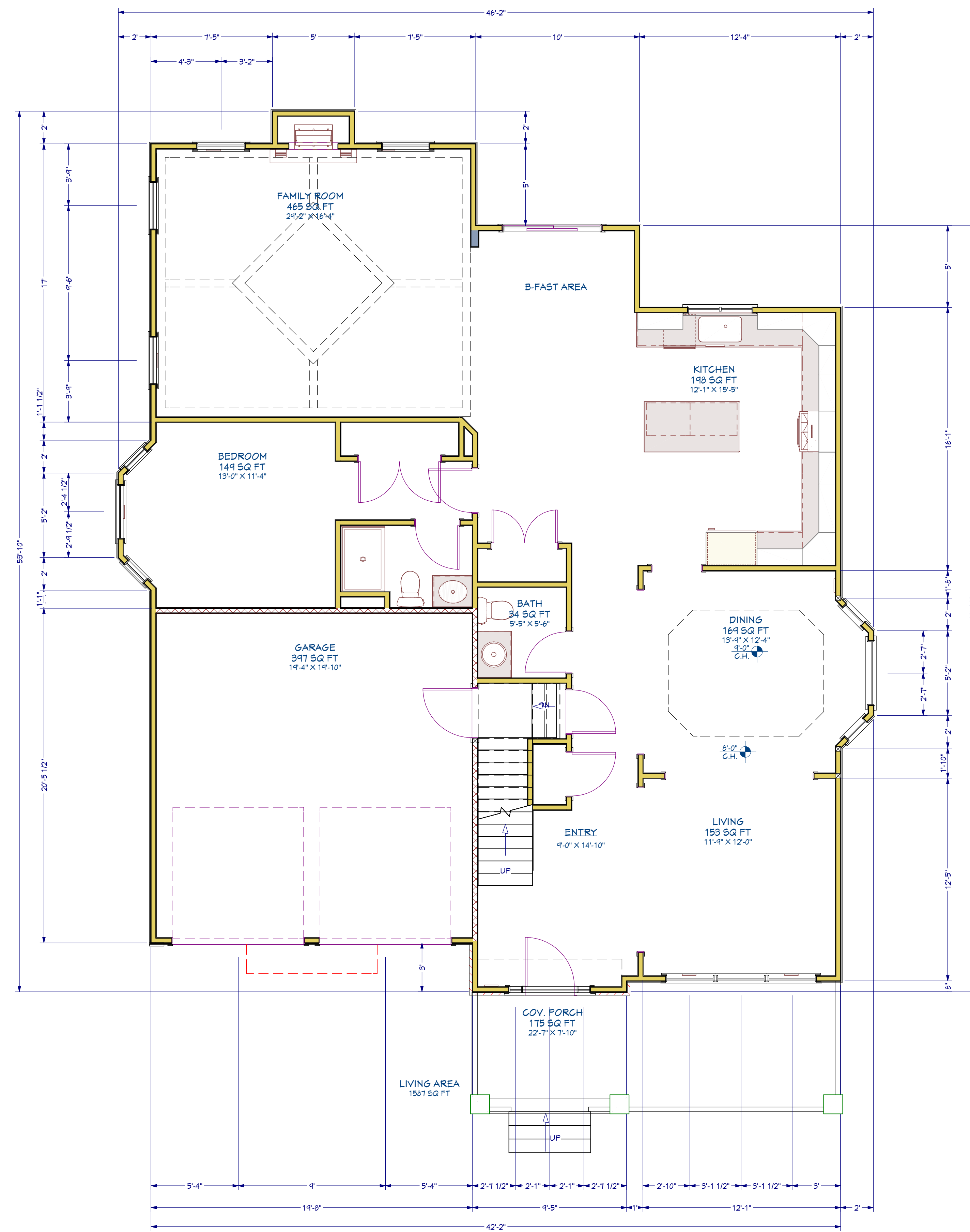
1st Floor 1/4 in = 1 ft
