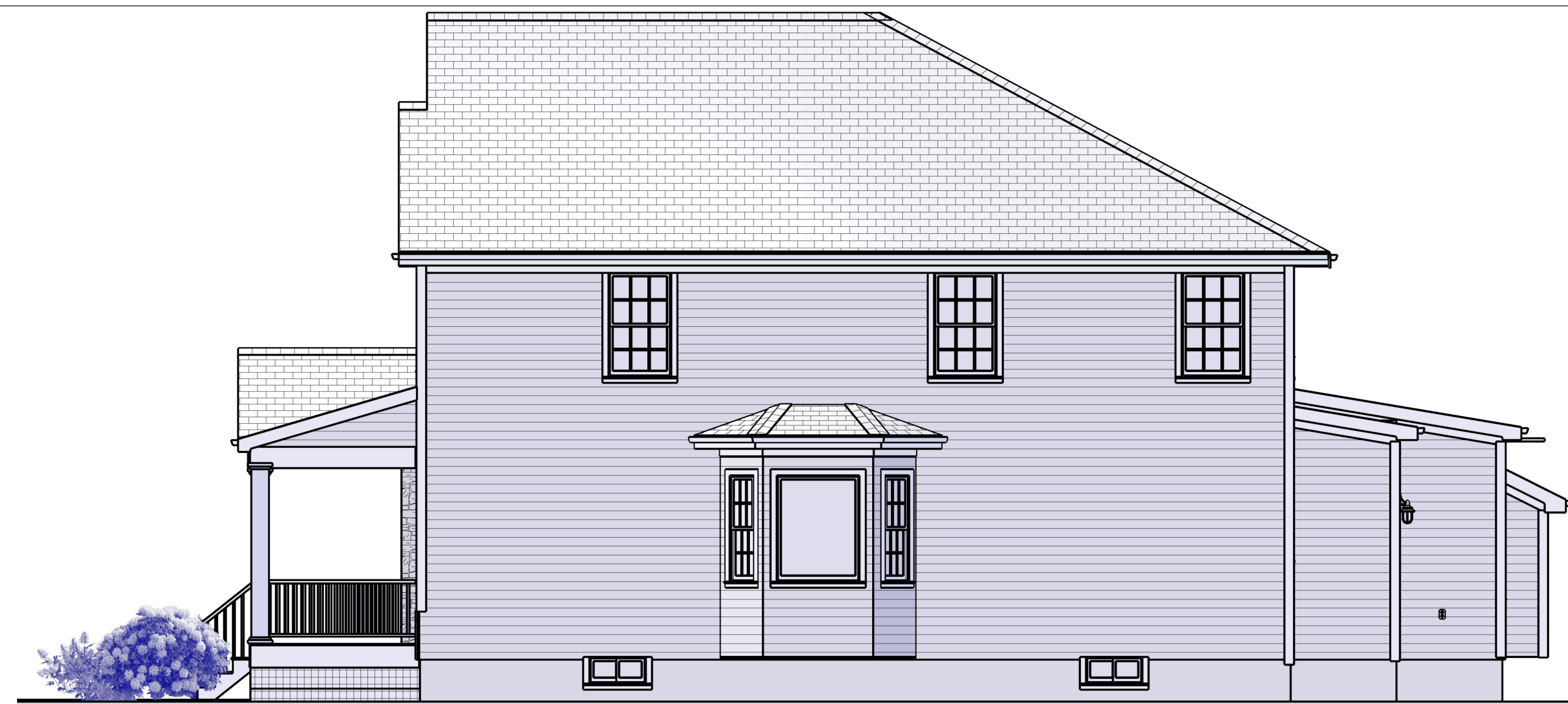
LEFT SIDE ELEVATION 3/16 in = 1 ft
